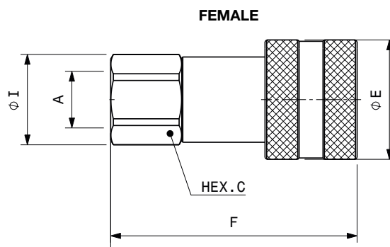
Female with internal thread
