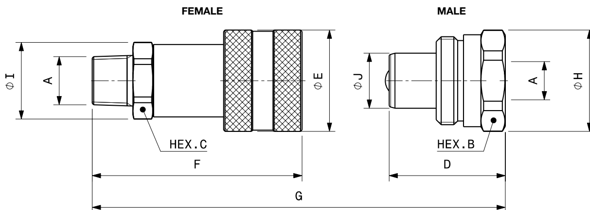
Female with external thread
