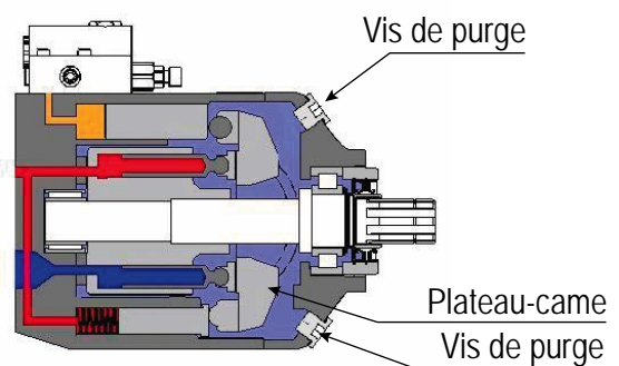
Figure 2 - Cylindrée nulle
